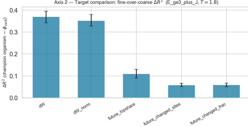
Figure 3: Target comparison ( T = 1.80 , predictor E_ge3_plus_J ). \Delta R^2 = \text{fine} - \text{coarse} across future targets. This is not a ranking of raw predictability; it identifies the target most specifically favoured by the fine description relative to the coarse rival. \Delta W achieves the largest fine advantage.
