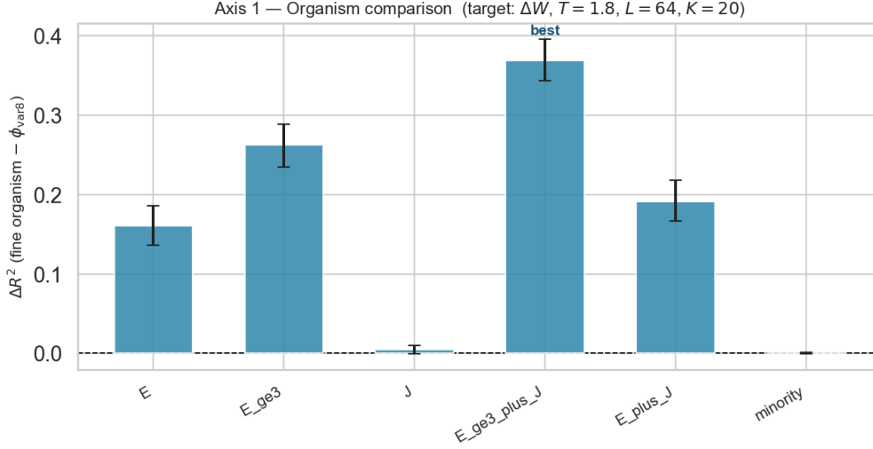
Figure 2: Organism comparison ( T = 1.80 , target \Delta W ). \Delta R^2 = R^2(\text{fine}) - R^2(\phi_{\text{var8}}) with bootstrap 95% CIs. Blue: fine wins; a red bar would indicate coarse wins. E_{\geq 3} + J (two-column model) achieves the largest advantage.
